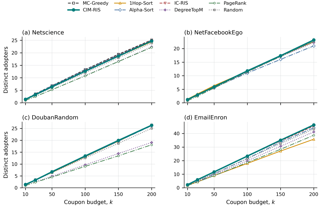
Figure 5: Adoption spread under the forwarding-heavy scenario. Longer forwarding paths increase the effect of graph structure, while low adoption probabilities also increase sampling variance.
