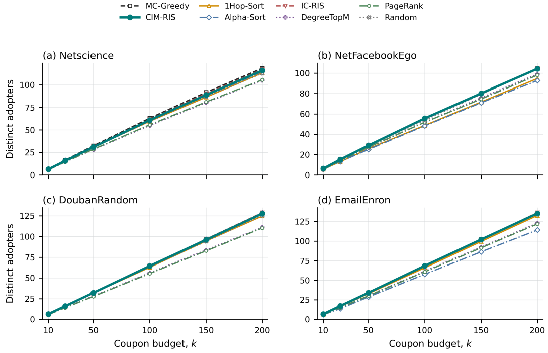
Figure 4: Adoption spread under the balanced scenario. Each point is evaluated using 10,000 fresh forward realizations. MC-Greedy is reported only on Netscience because it estimates a full source-adopter probability matrix.
