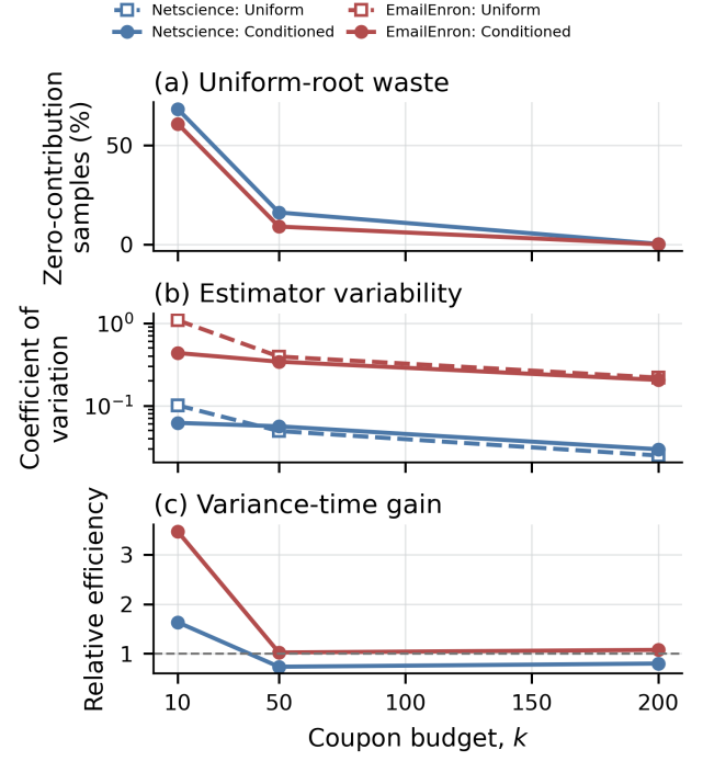
Figure 6: Uniform-root versus conditioned-root estimation in the forwarding-heavy scenario. Each statistic uses 30 independent batches of 20,000 samples. Relative efficiency is the ratio of the variance-time products of uniform and conditioned sampling; values above one favor conditioning.
