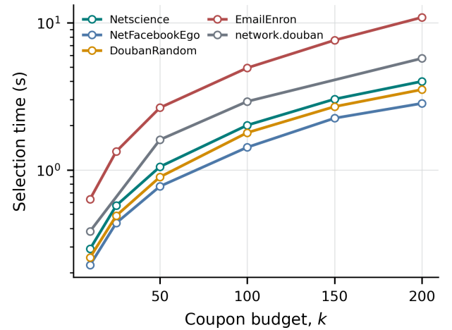
Figure 7: Single-process CIM-RIS selection time in the balanced scenario with 10,000 joint RR samples on five graph instances.
